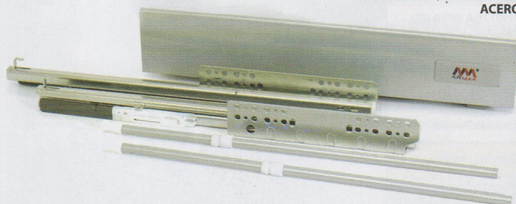
RIEL EXTENSIÓN TOTAL REF. SH4501J-35 REF. SH4501J-45 REF. SH4501J-40 REF. SH4501J-50 ACERO ENDURECIDO
